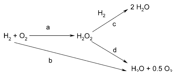
Scheme 1. Formation and decomposition pathways for hydrogen peroxide. a) Formation, b) combustion, c) hydrogenation, and d) decomposition.
